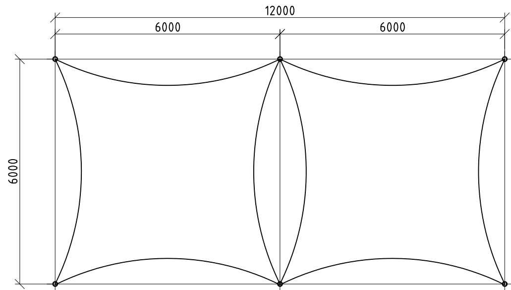
PLAN - 12m x 6m
