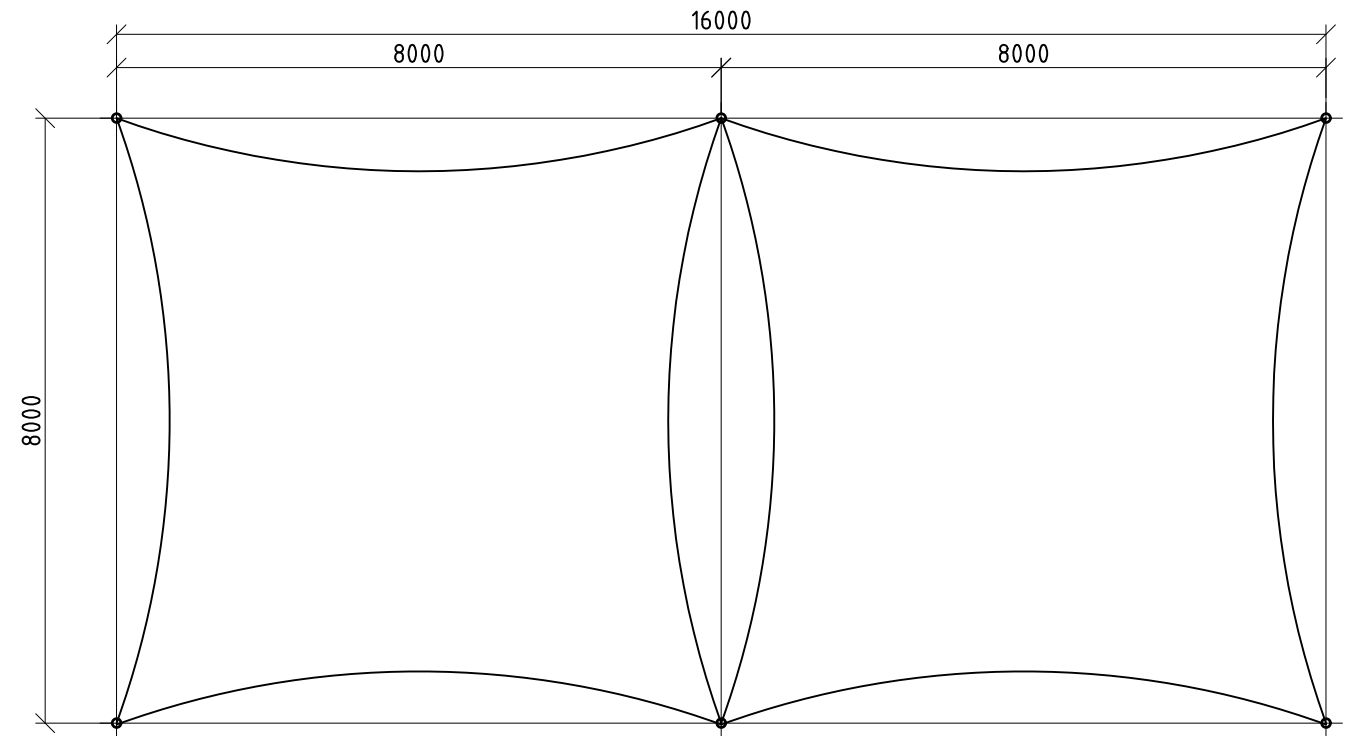
PLAN - 16m x 8m
