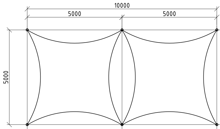
PLAN - 10m x 5m
