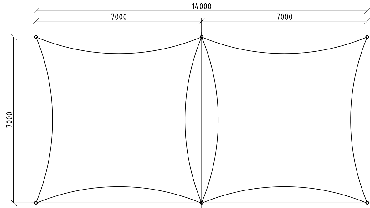
PLAN - 14m x 7m
