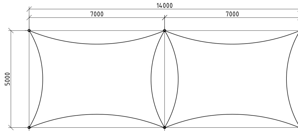
PLAN - 14m x 5m
