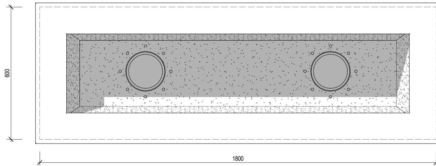
3 PLAN 001 1:10 @ A3
