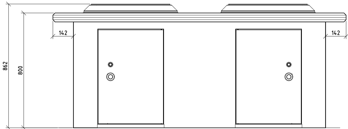
2 FRONT ELEVATION SCALE (1:15)
