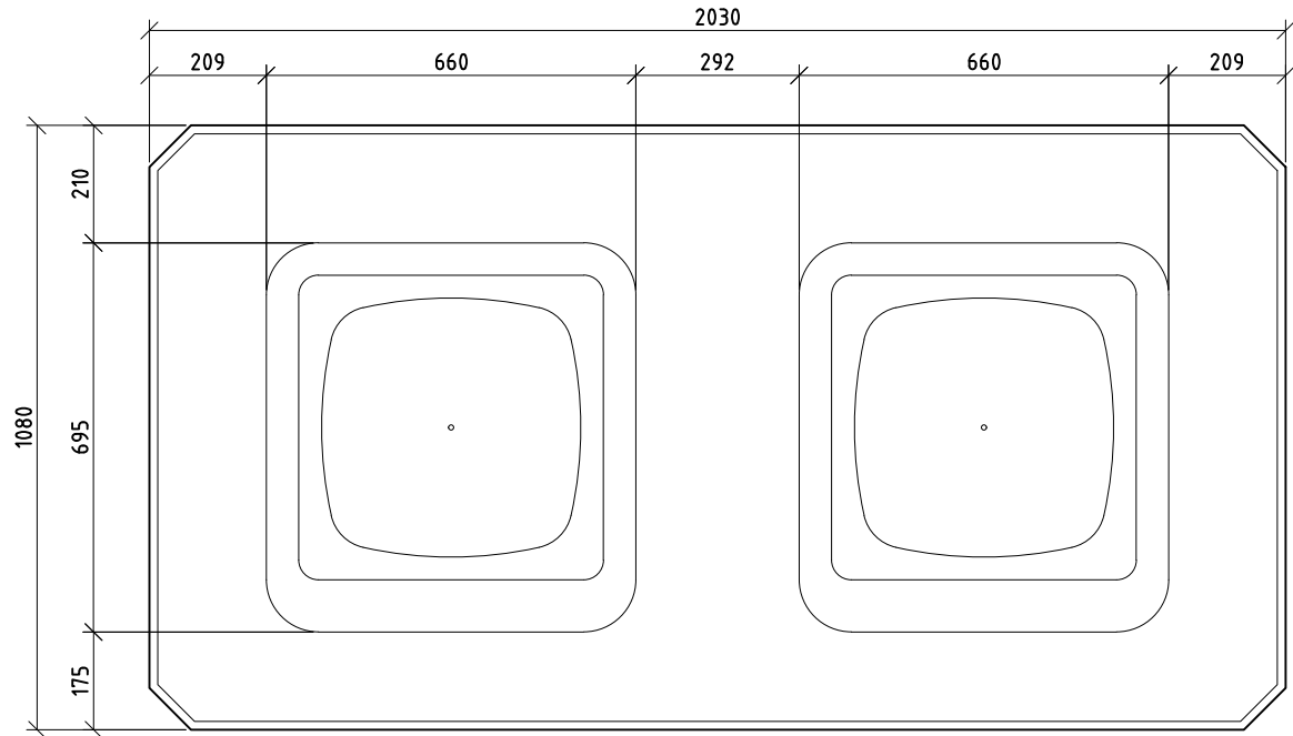
1 PLAN SCALE (1:15)
