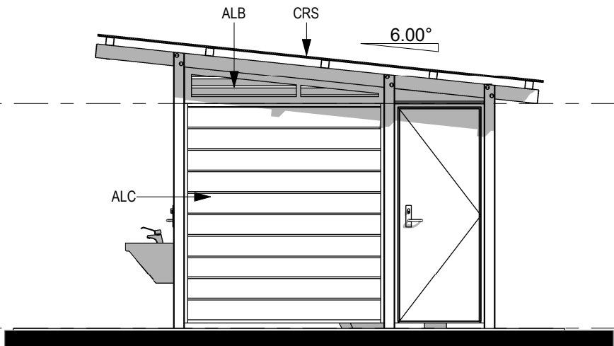
3 ELEVATION SIDE 001 1 : 50 @ A3
