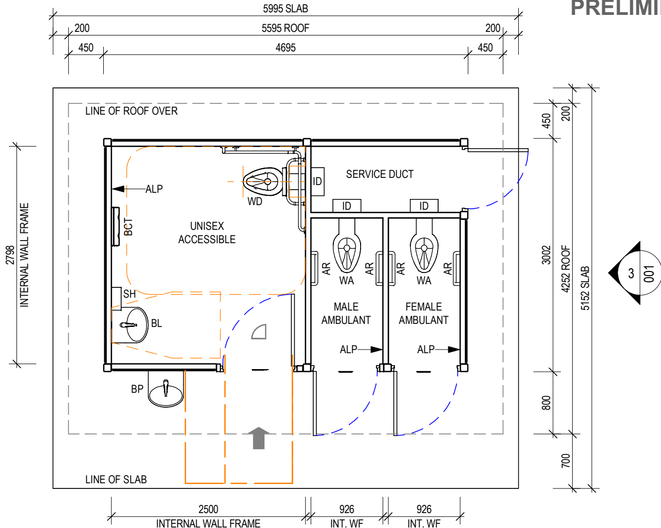
1 FLOOR PLAN 001 1 : 50 @ A3
