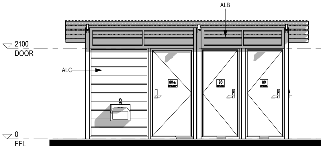
2 ELEVATION FRONT 001 1 : 50 @ A3
