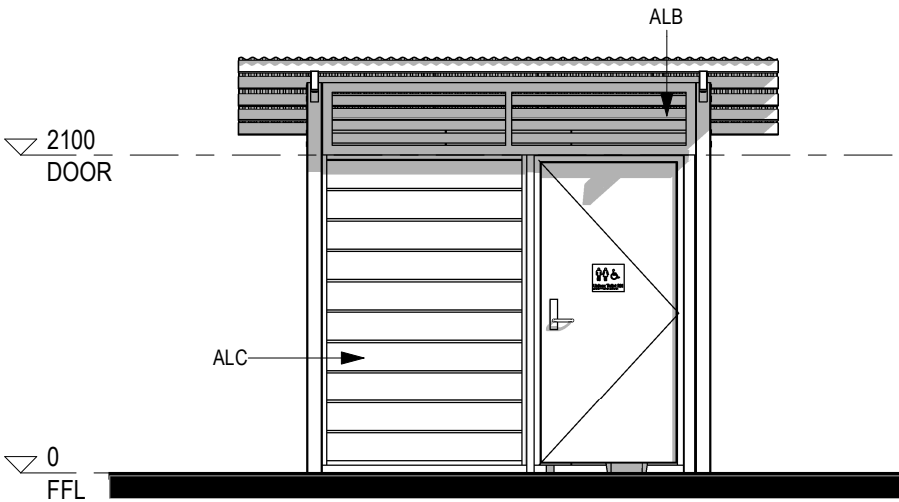
2 ELEVATION FRONT 1 : 50 @ A3
