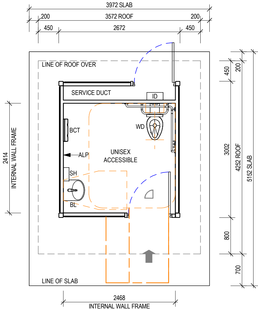
1 FLOOR PLAN 001 1 : 50 @ A3
