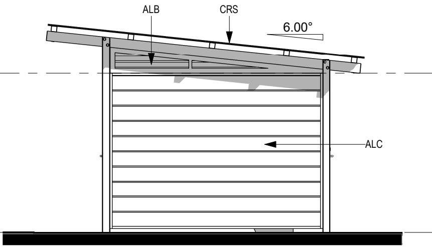
3 ELEVATION SIDE 1 : 50 @ A3
