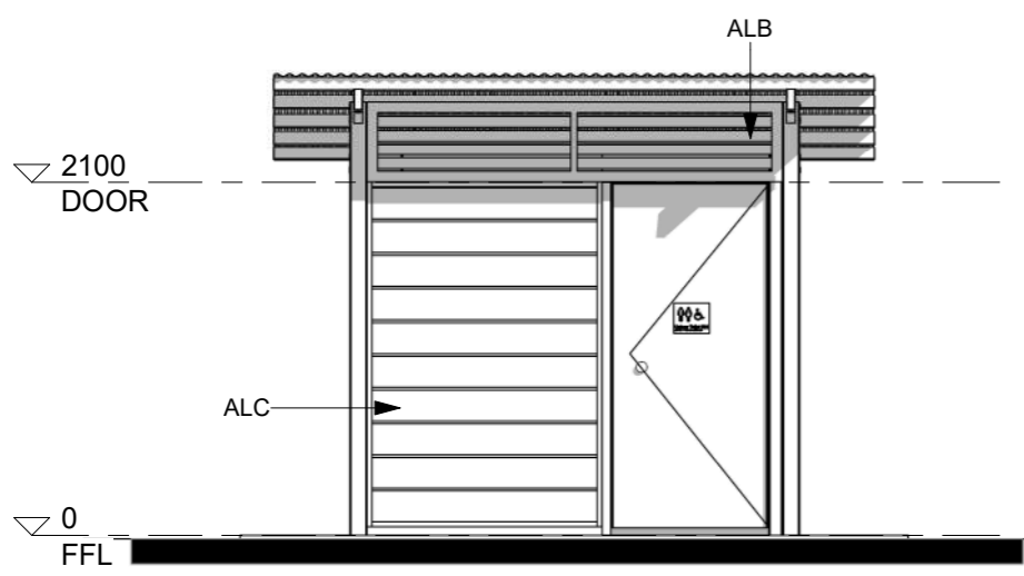
2 ELEVATION FRONT 001 1 : 50 @ A3
