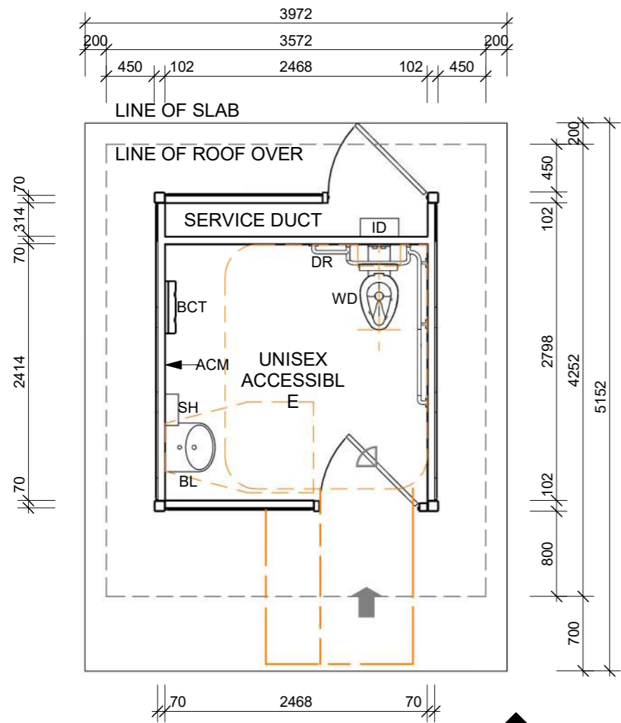
1 FLOOR PLAN 001 1 : 50 @ A3
