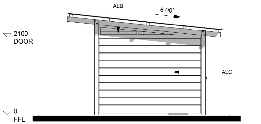
3 ELEVATION SIDE 001 1 : 50 @ A3
