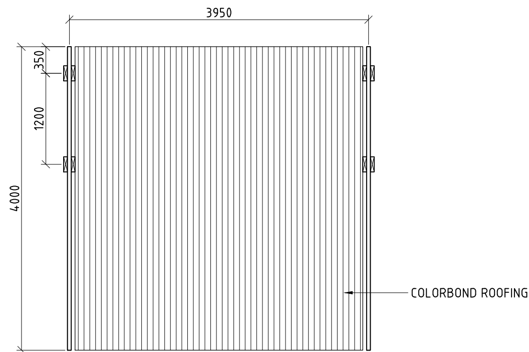
PLAN SCALE (1:50)
