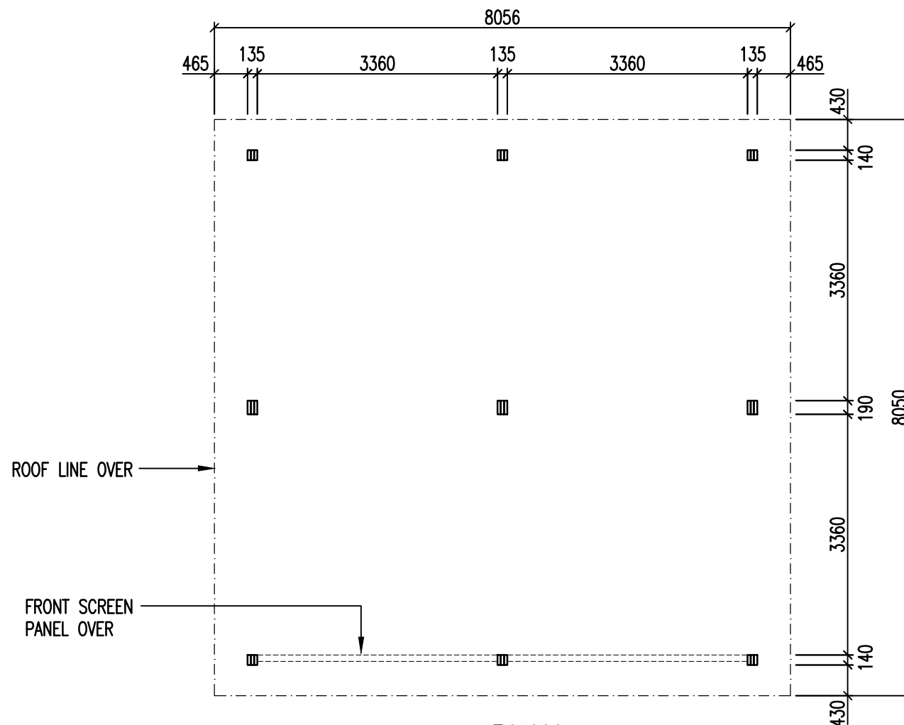
PLAN
