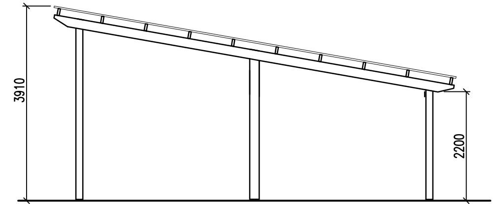
SIDE ELEVATION
