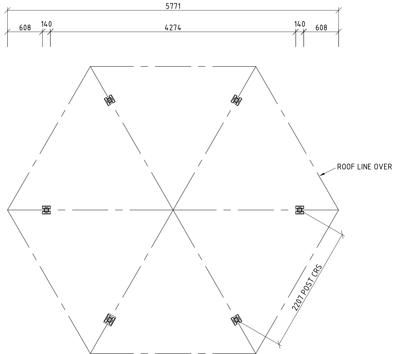
PLAN SCALE (1:40)
