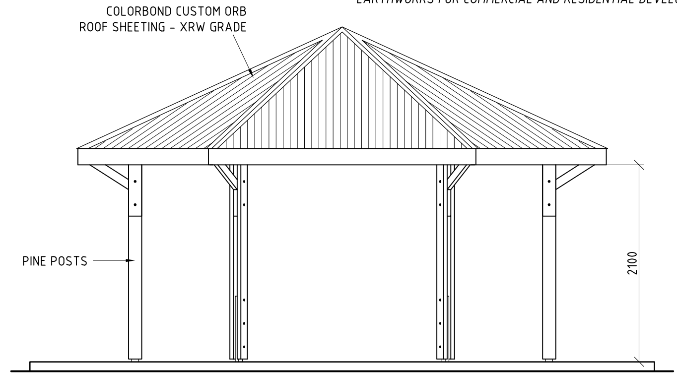
ELEVATION SCALE (1:40)
