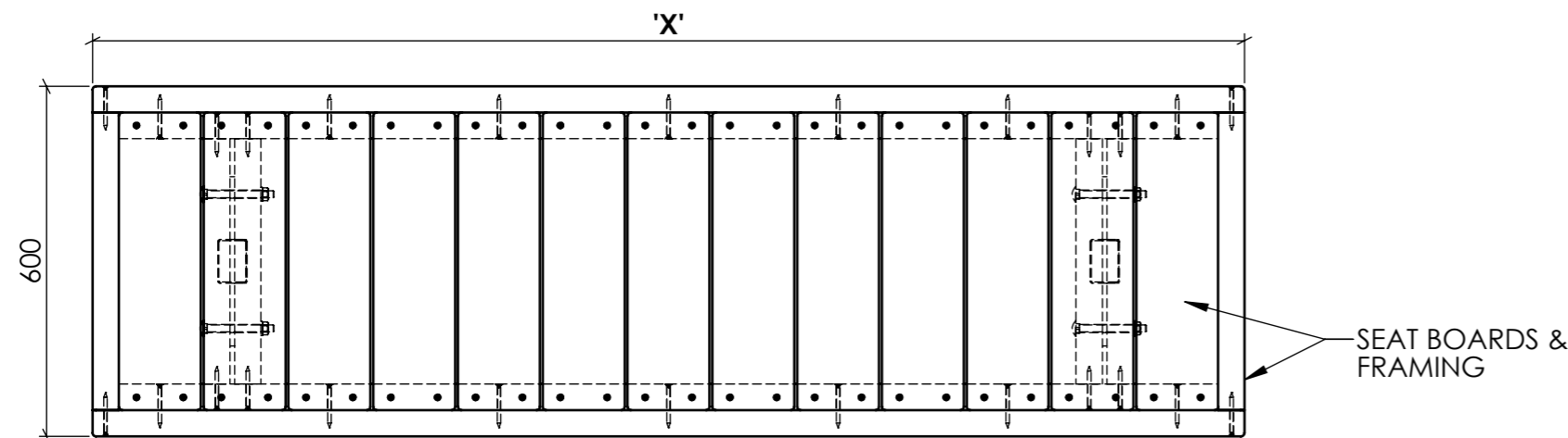
TOP VIEW
