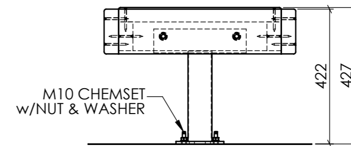
SIDE VIEW (BOLT DOWN)
