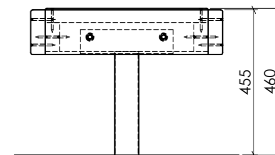
SIDE VIEW (IN-GROUND)
