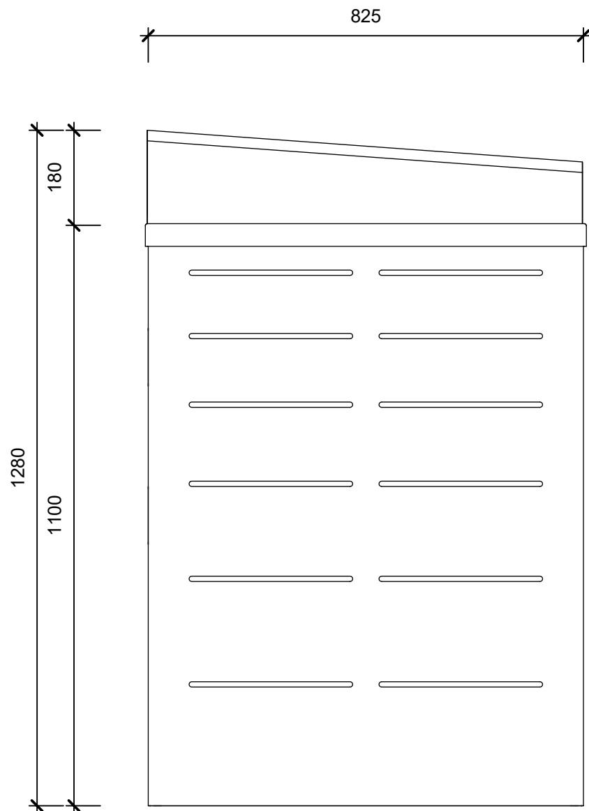
SIDE ELEVATION
