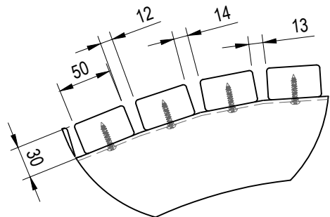
DETAIL-A (1:5)
