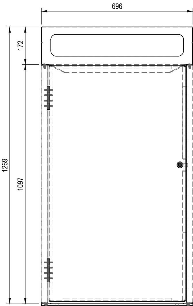
FRONT VIEW
