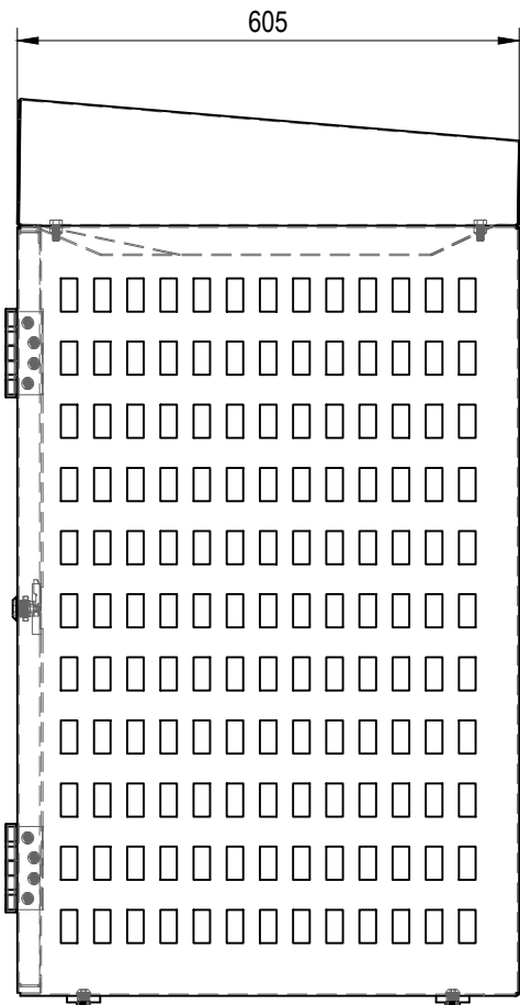
SIDE VIEW
