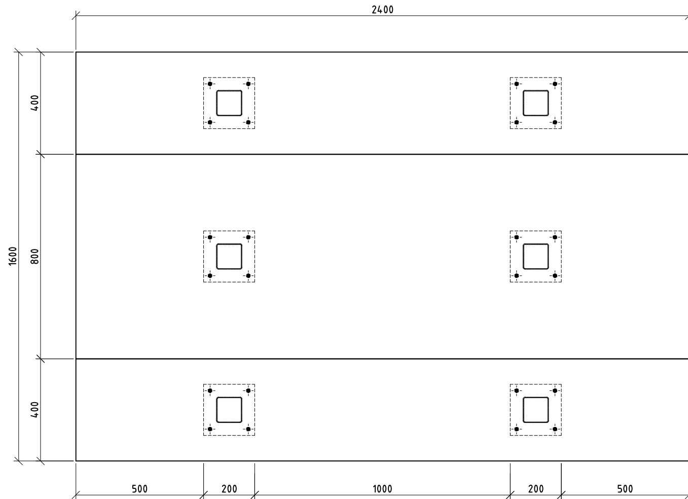
1 PLAN 1:15 @ A3
