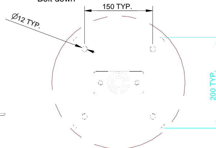
Detail A TYPICAL BOLT DOWN DETAIL TIMBER SLATS REMOVED FOR CLARRITY
