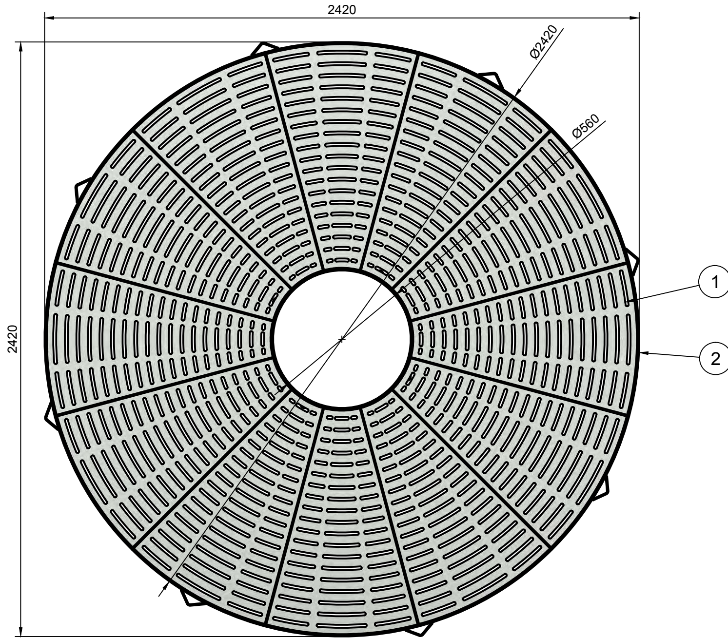
PLAN VIEW
