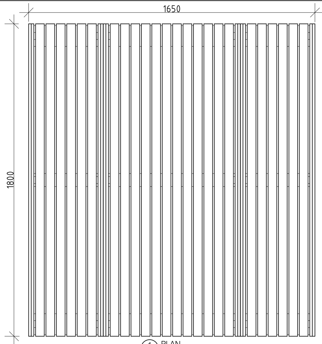
1 PLAN 1:15 @ A3 1650
