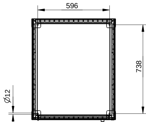
BOLT DOWN DETAIL
