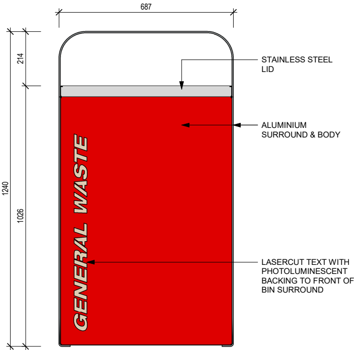
2 ELEVATION FRONT 1 : 15 @ A3
