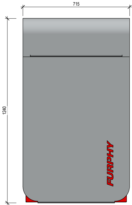
3 ELEVATION LEFT 1 : 15 @ A3
