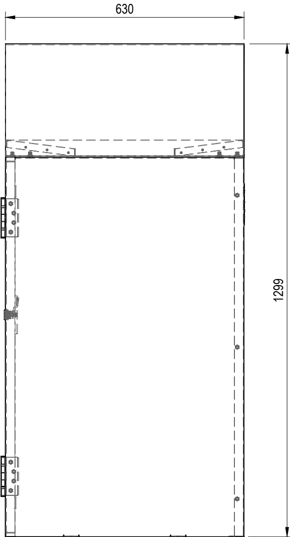
END VIEW
