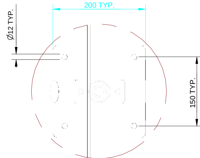
Detail A SLATS REMOVED FOR CLARITY
