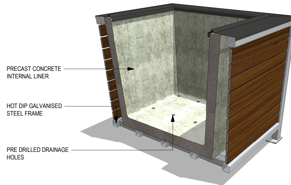
1 SECTIONAL PERSPECTIVE @ A3
