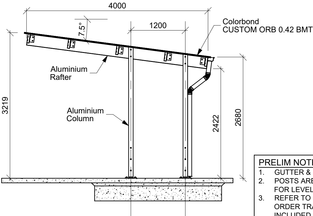
SECTION A 1:50
