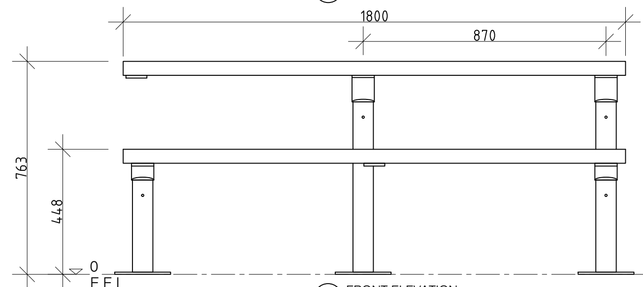
3 FRONT ELEVATION 1:15 @ A3
