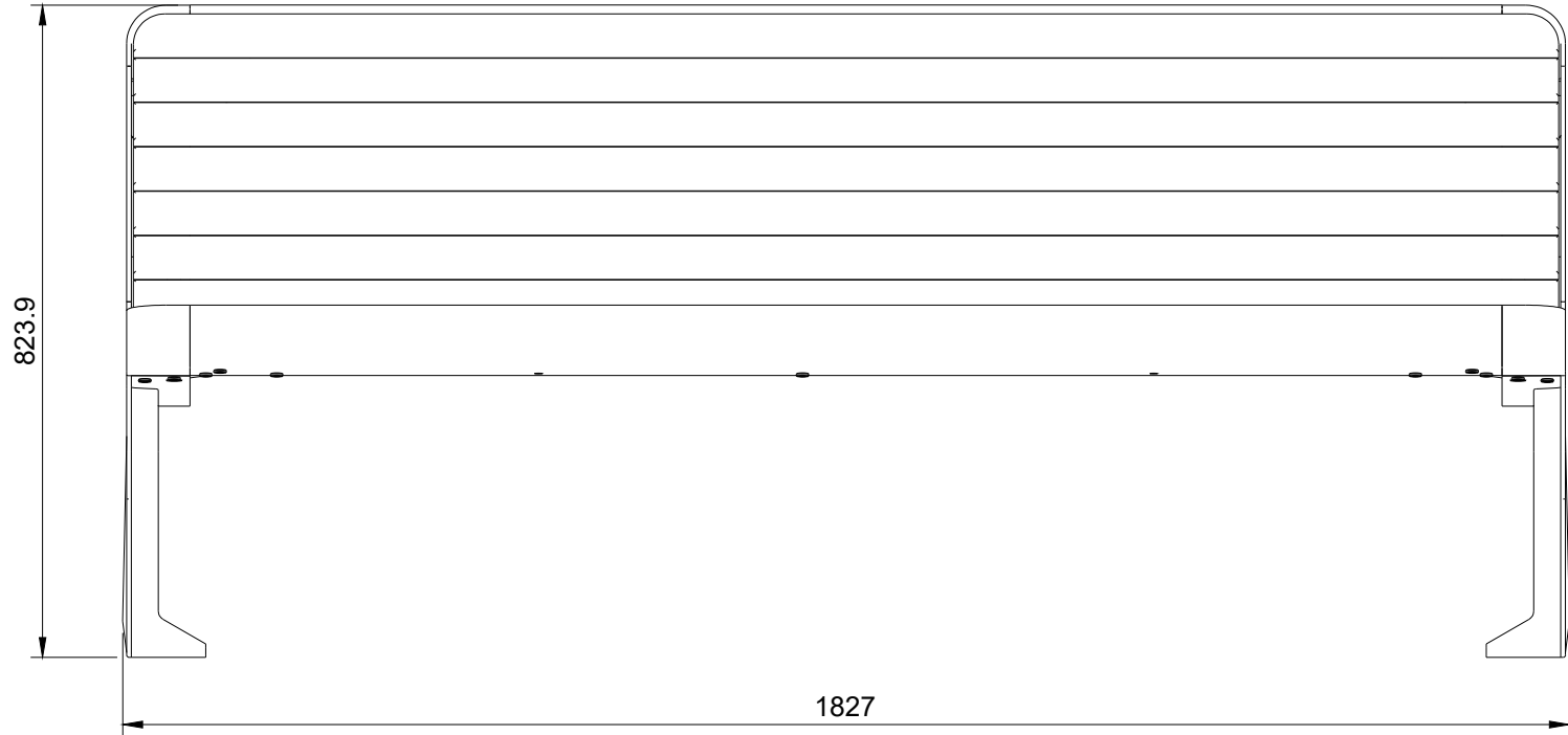
FRONT VIEW
