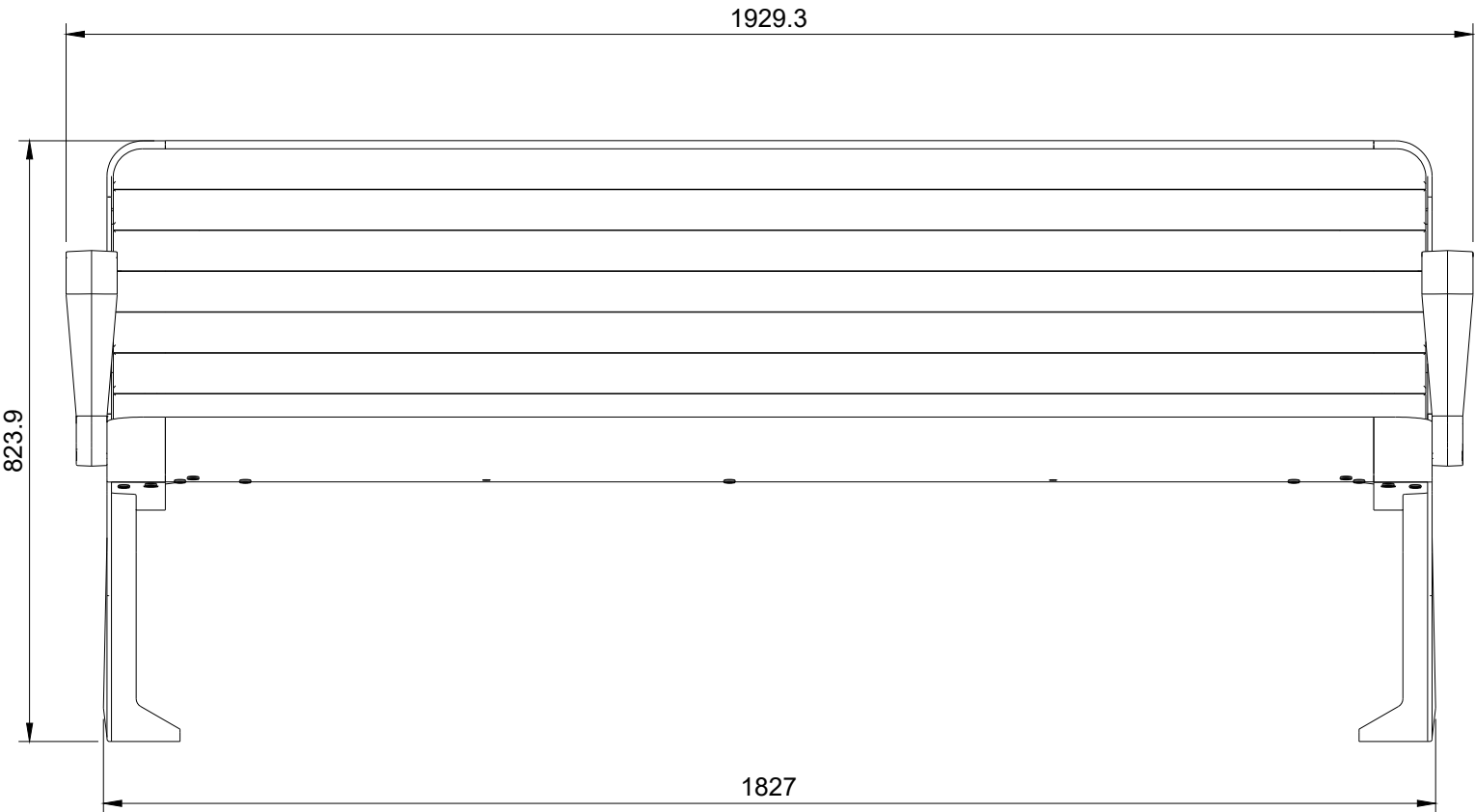
FRONT VIEW
