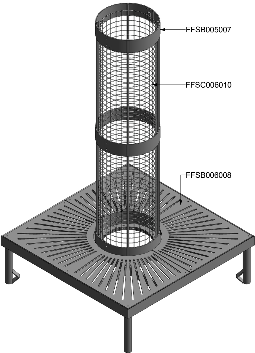
3 ISOMETRIC VIEW
