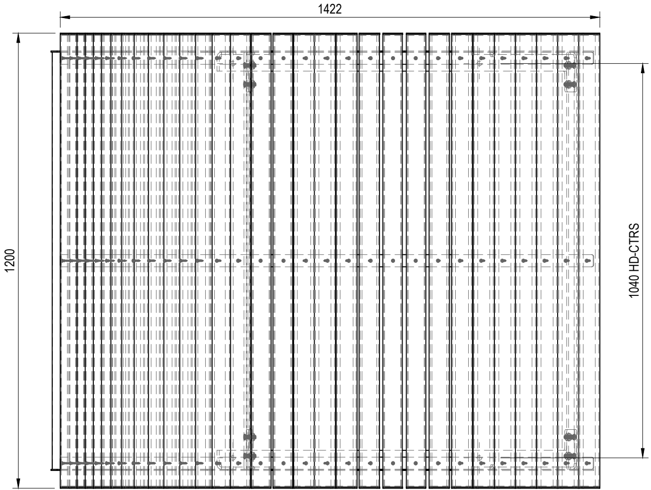
TOP VIEW
