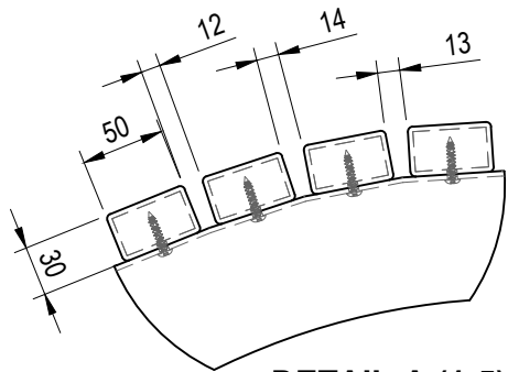
DETAIL-A (1:5) GAPS VARY DUE TO CURVITURE
