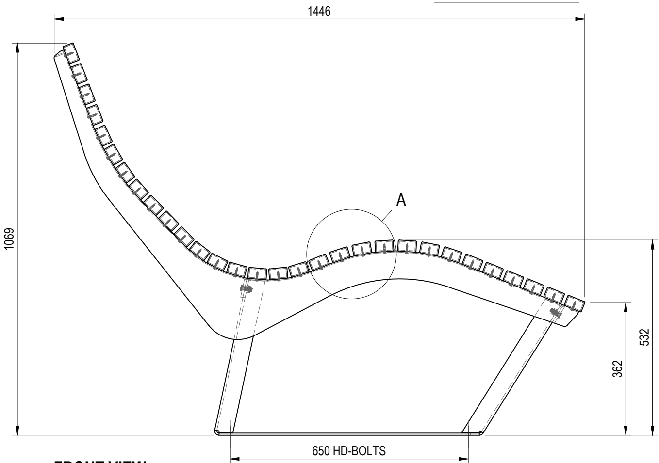
FRONT VIEW
