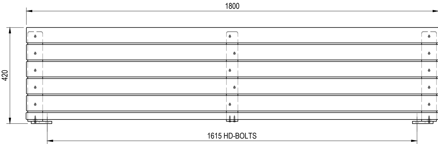
FRONT VIEW
