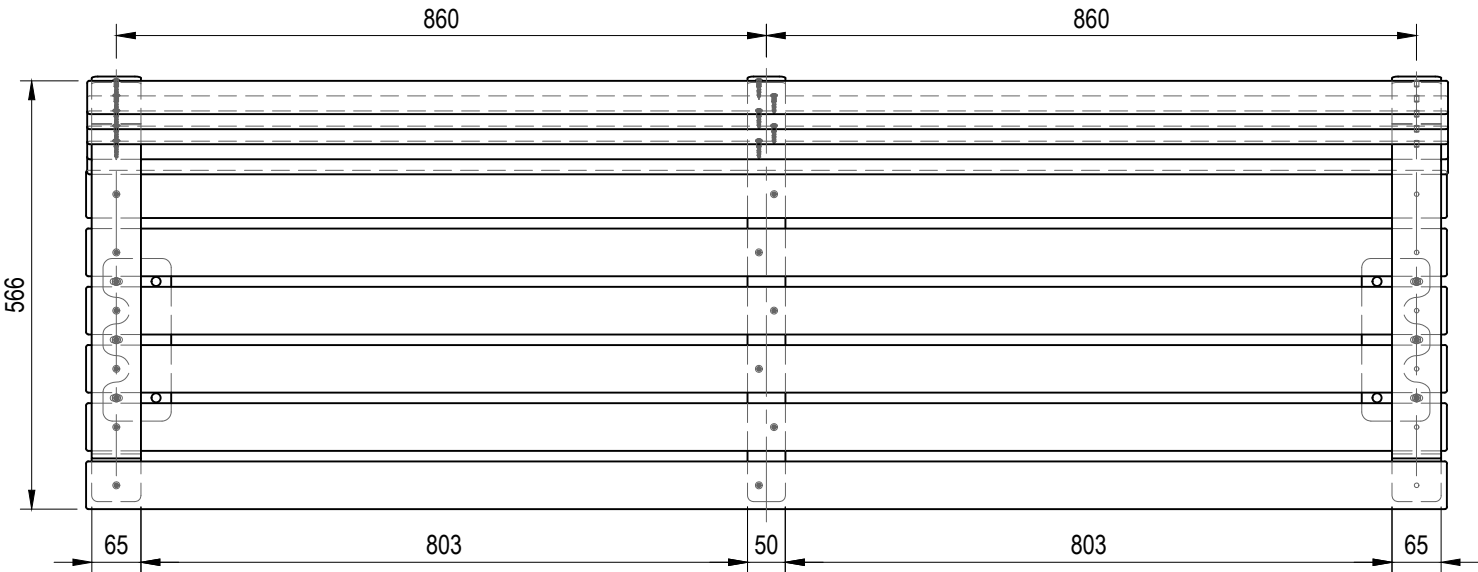
TOP VIEW
