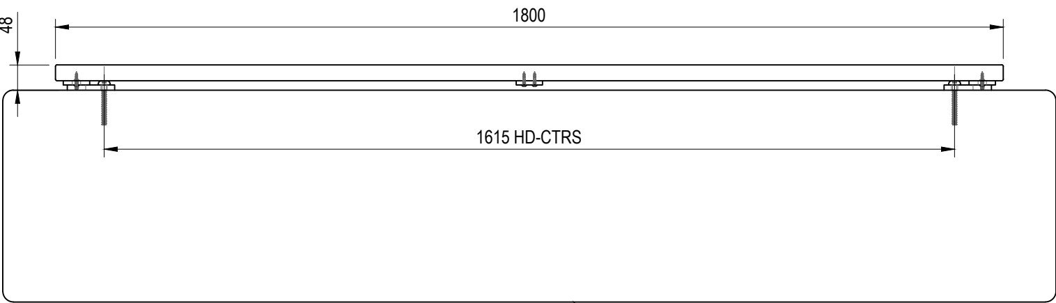
FRONT VIEW
