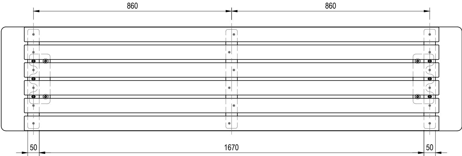
TOP VIEW
