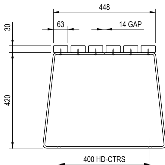
END VIEW
