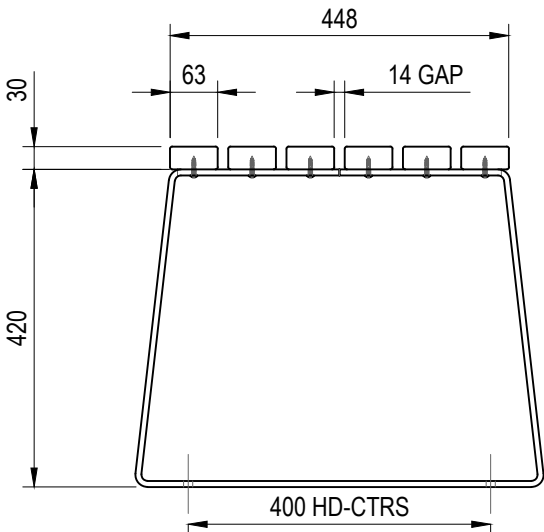
END VIEW
