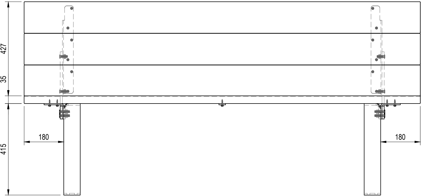
FRONT VIEW
