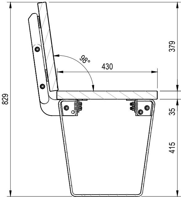
SECTION A-A (1:10)
