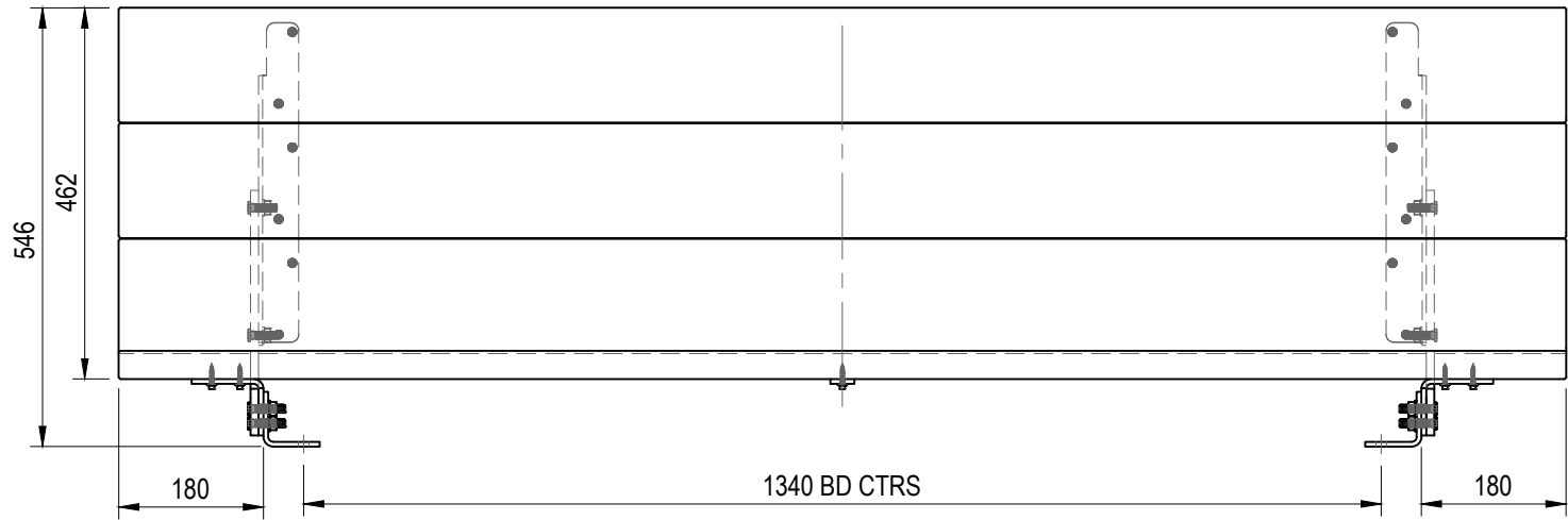
FRONT VIEW
