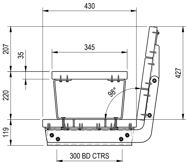
END VIEW
