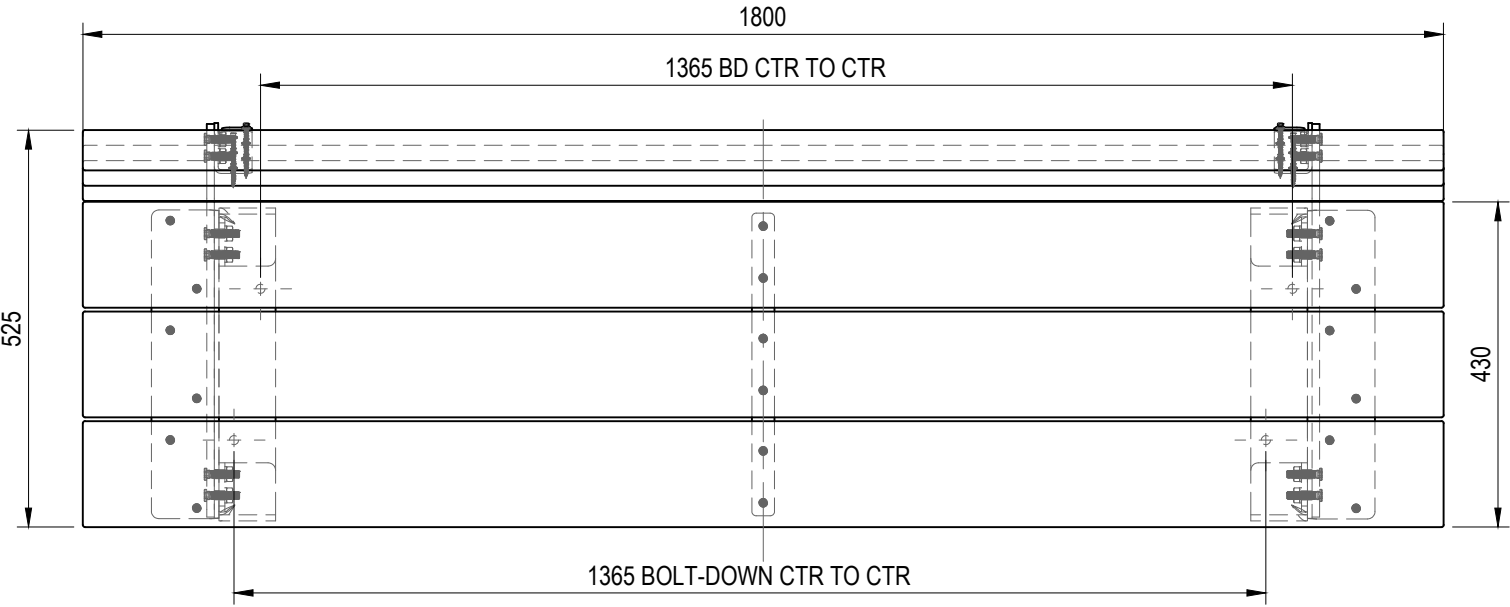
TOP VIEW
