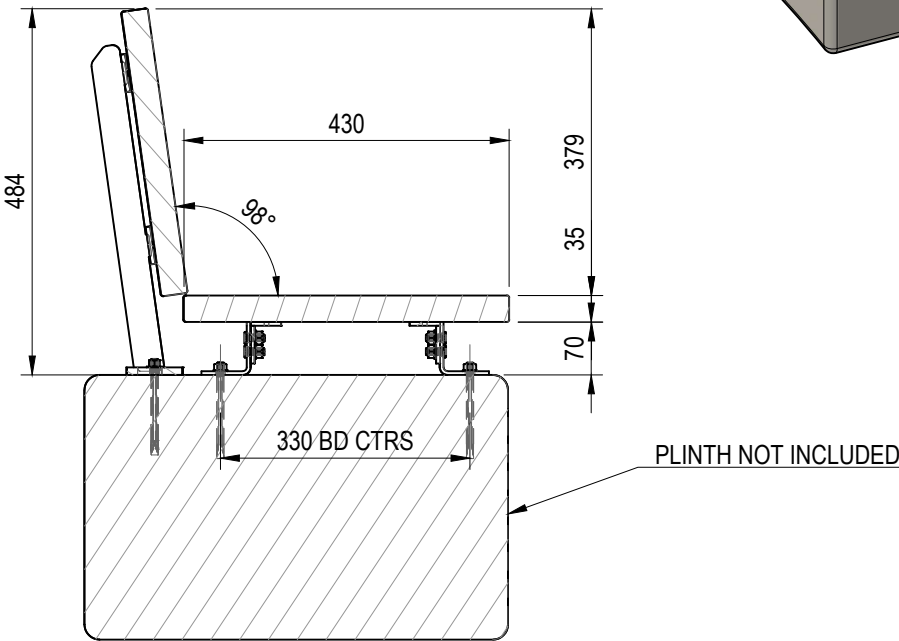
SECTION A-A (1:10)
