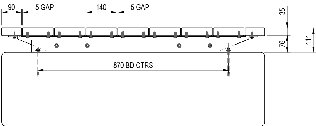
END VIEW
