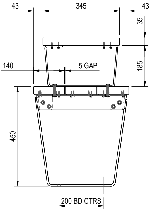
END VIEW
