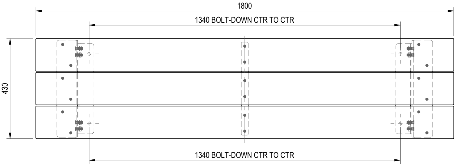
TOP VIEW
