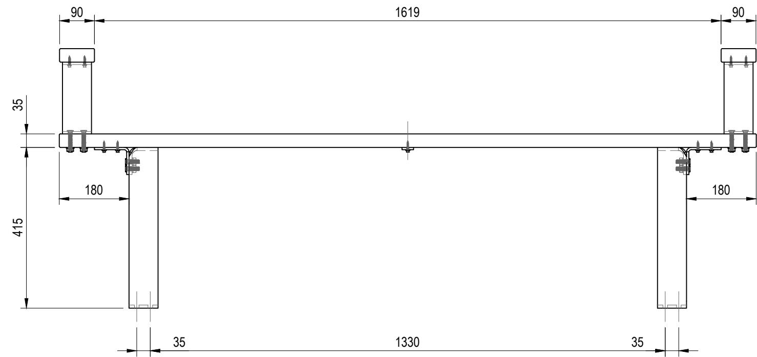
FRONT VIEW
