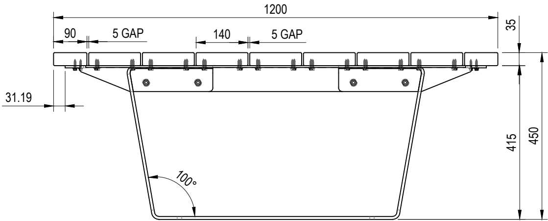
SIDE VIEW
