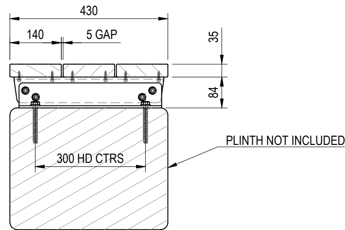
SECTION A-A (1:10)
