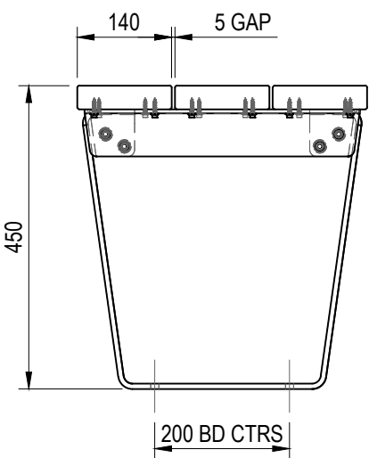
END VIEW
