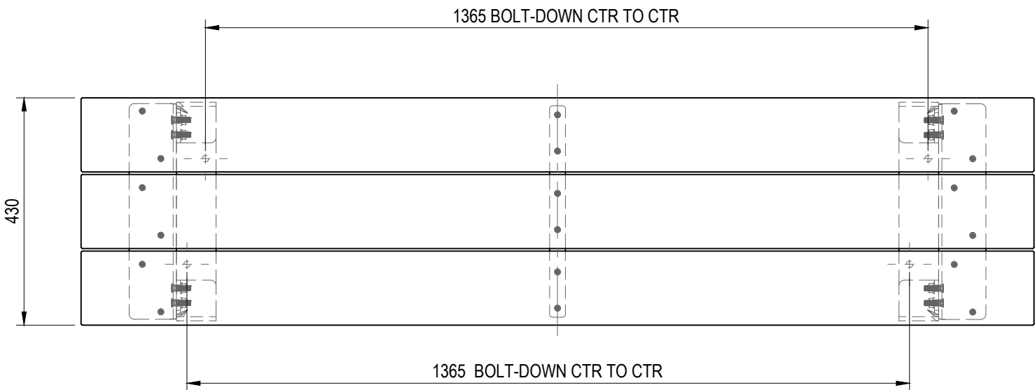
TOP VIEW
