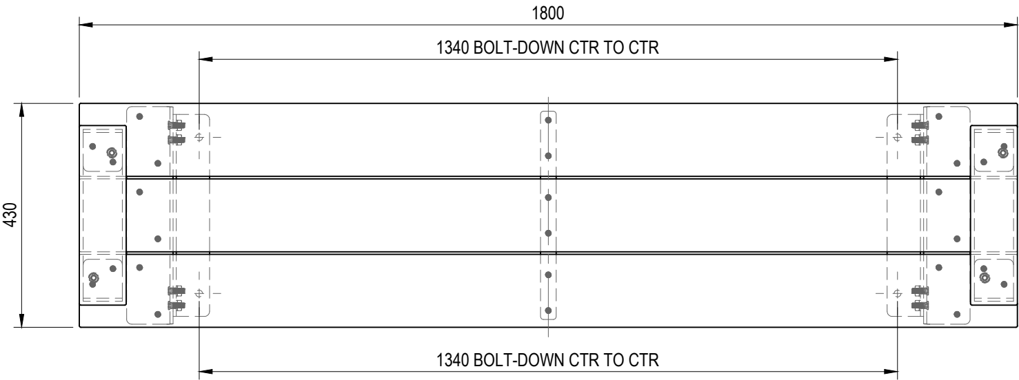
TOP VIEW
