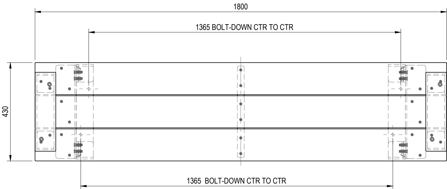
TOP VIEW
