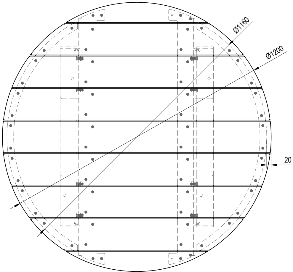
TOP VIEW
