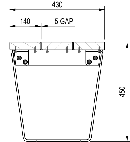
SECTION A-A (1:10)
