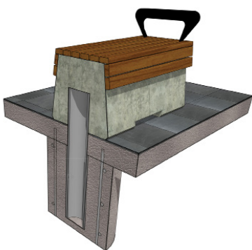
Typical steel reinforced fixing pin installation
